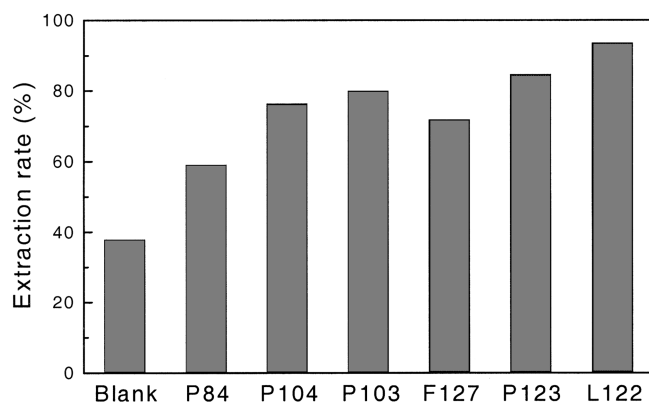
Fig. 5. The extraction rates of hydrogel at 22 °C; the hydrogel was composed of 5 wt% alginate gel and 2 wt% Pluronic copolymer.
